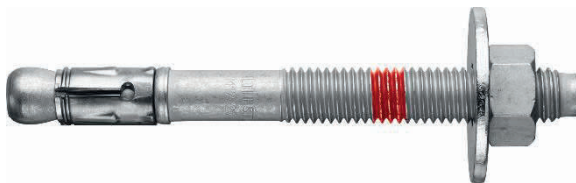
HST3-BW HST3-R-BW (M8-M24)
